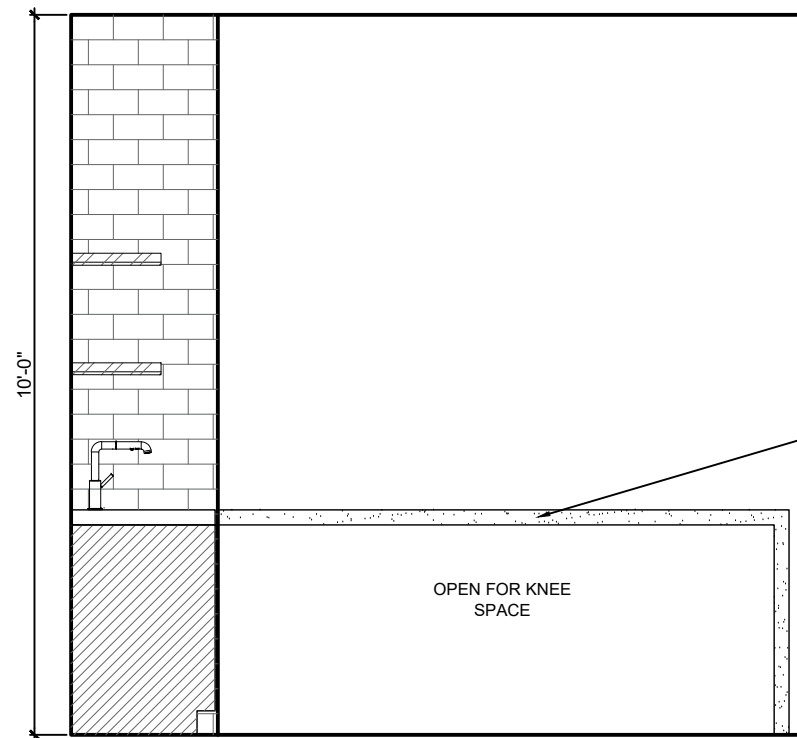
104 BAR - ELEVATION C
