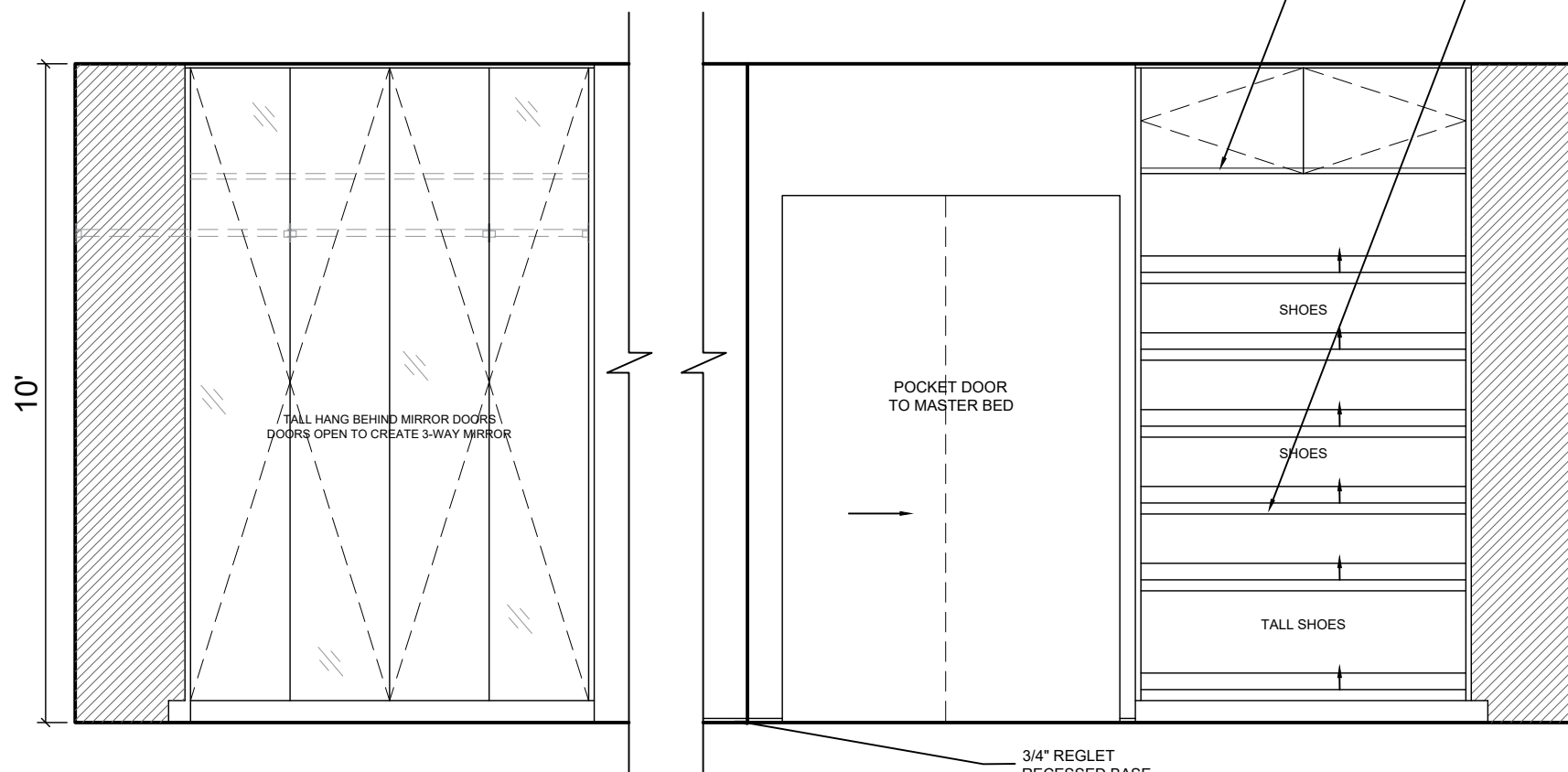
203 MASTER W.I.C - ELEVATION A
