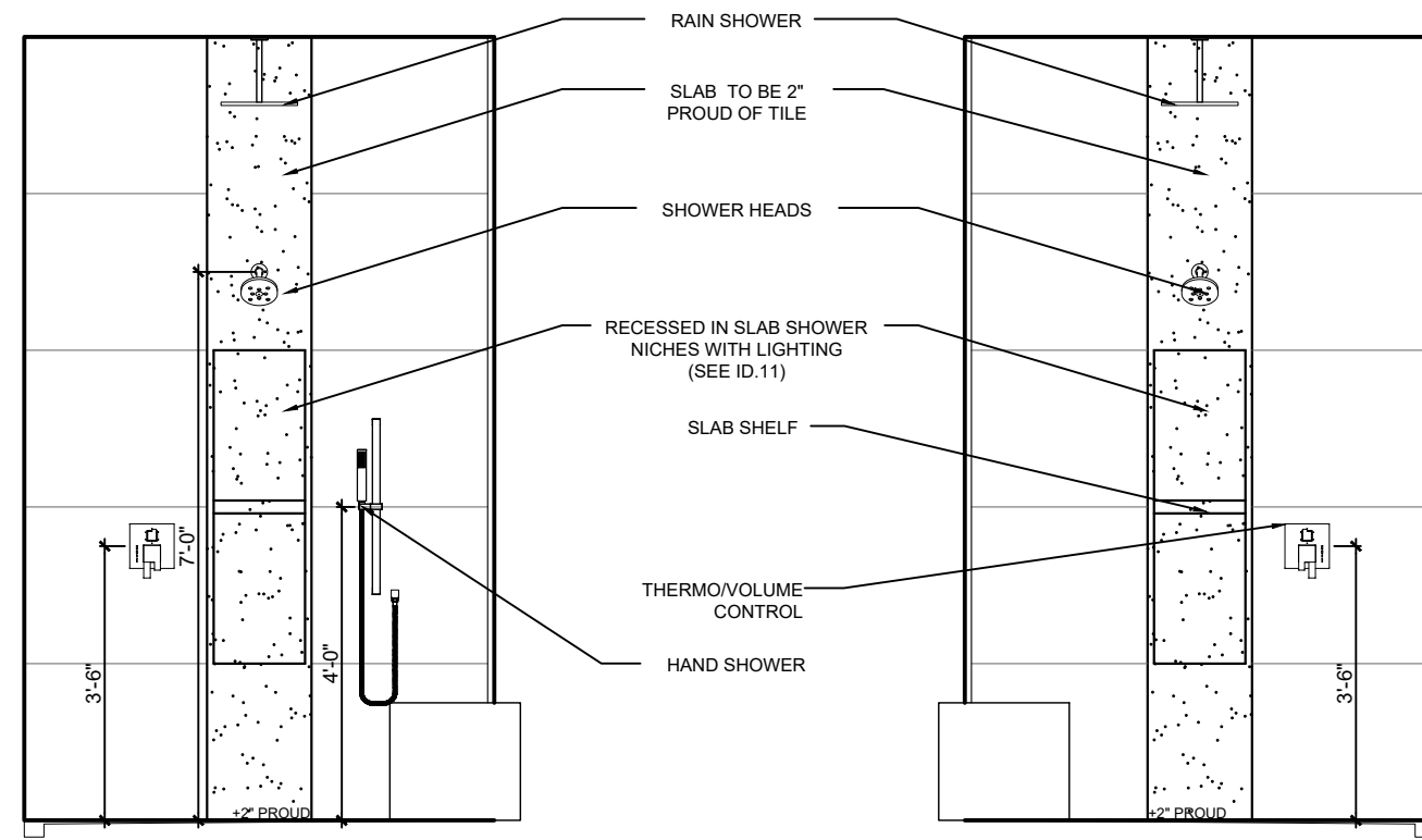
202 MASTER BATH - SHOWER ELEVATION B
