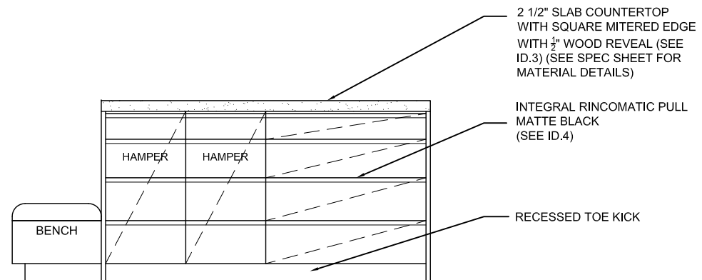
203 MASTER W.I.C - ISLAND - ELEVATION A
