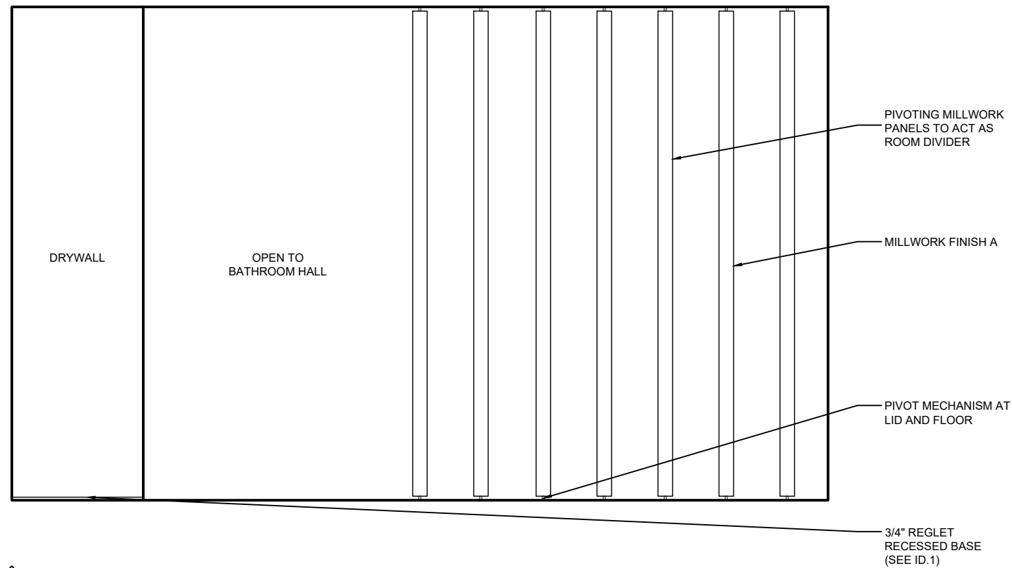
201 MASTER BEDROOM ELEVATION A
