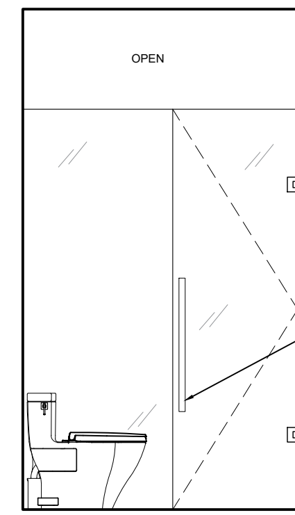
112 BATH 2 - ELEVATION B
