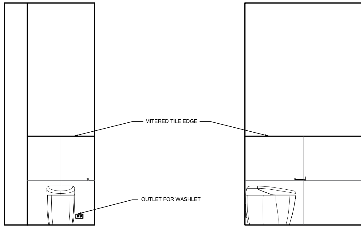
202 MASTER BATH - WC 2 ELEVATION A
