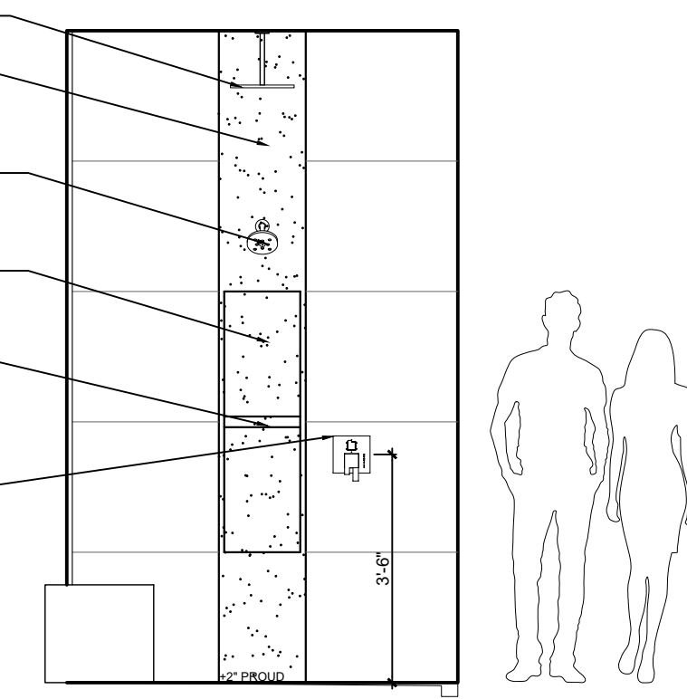
202 MASTER BATH - SHOWER ELEVATION C
