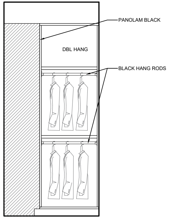
111 W.I.C 1 - ELEVATION B
