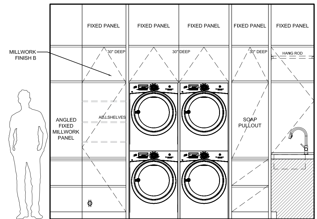
116 LAUNDRY - ELEVATION C
