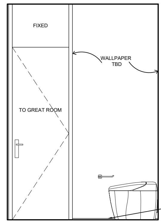
108 POWDER - ELEVATION C
