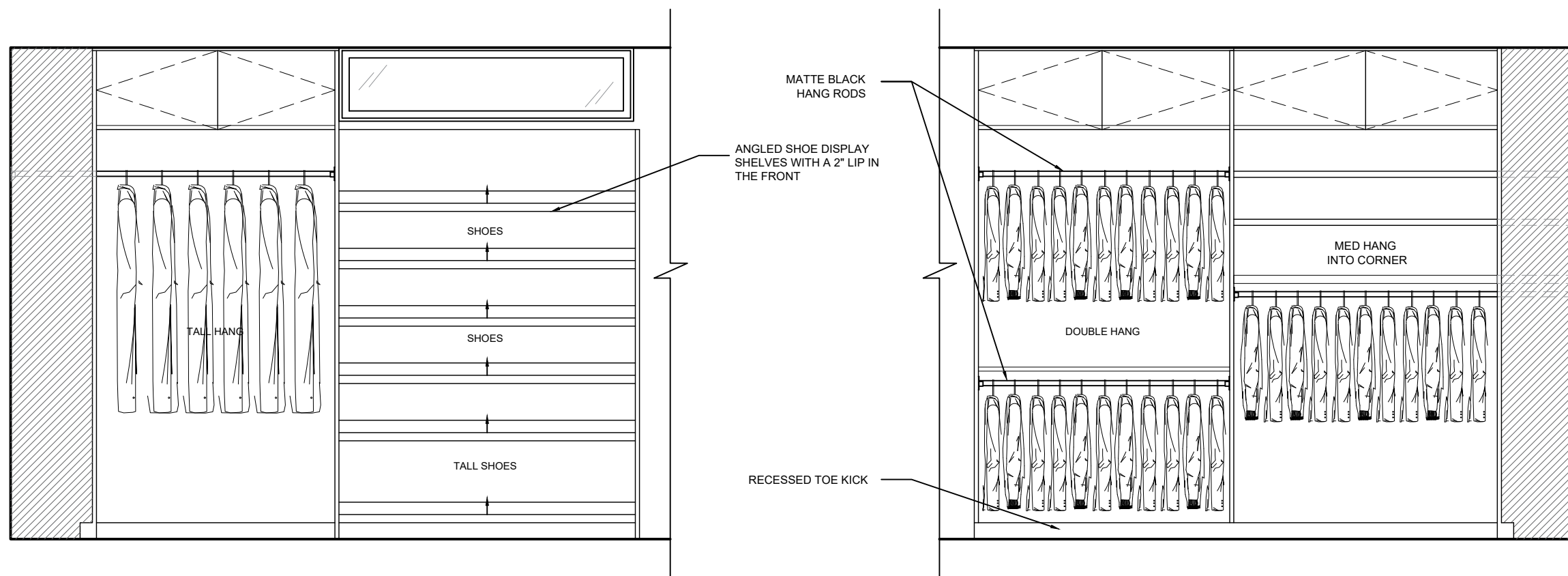
203 MASTER W.I.C - ELEVATION C
