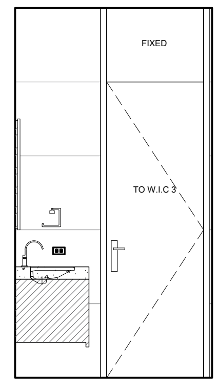
114 BATH 3 - ELEVATION D
