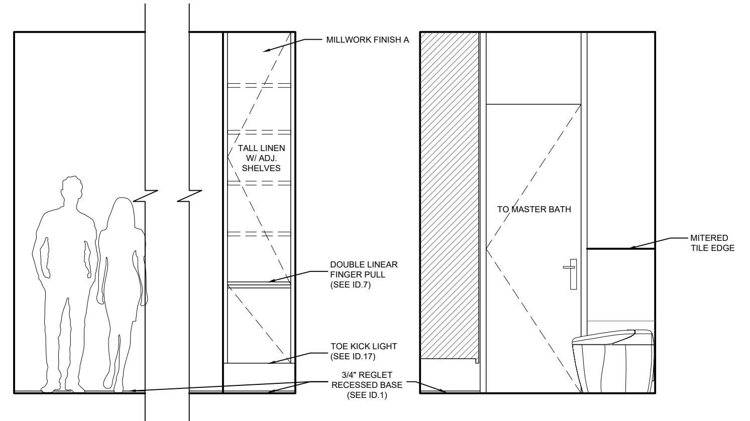
202 MASTER BATH - WC 2 ELEVATION C
