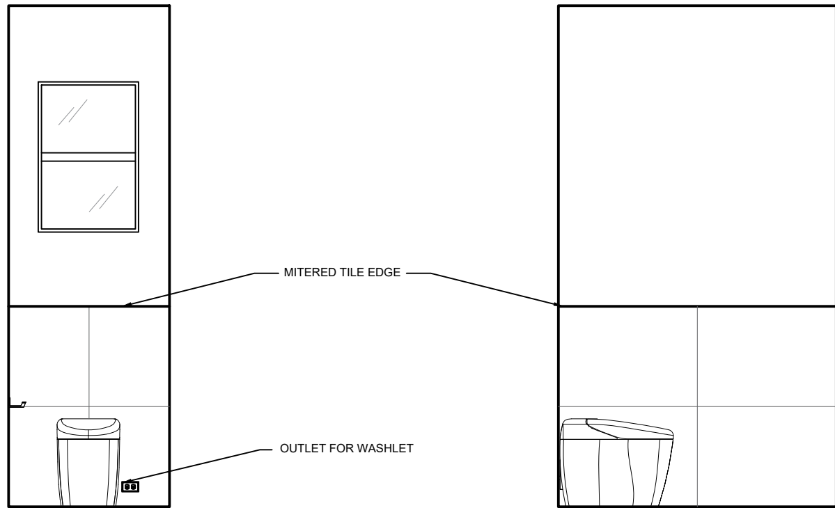
202 MASTER BATH - WC 1 ELEVATION A
