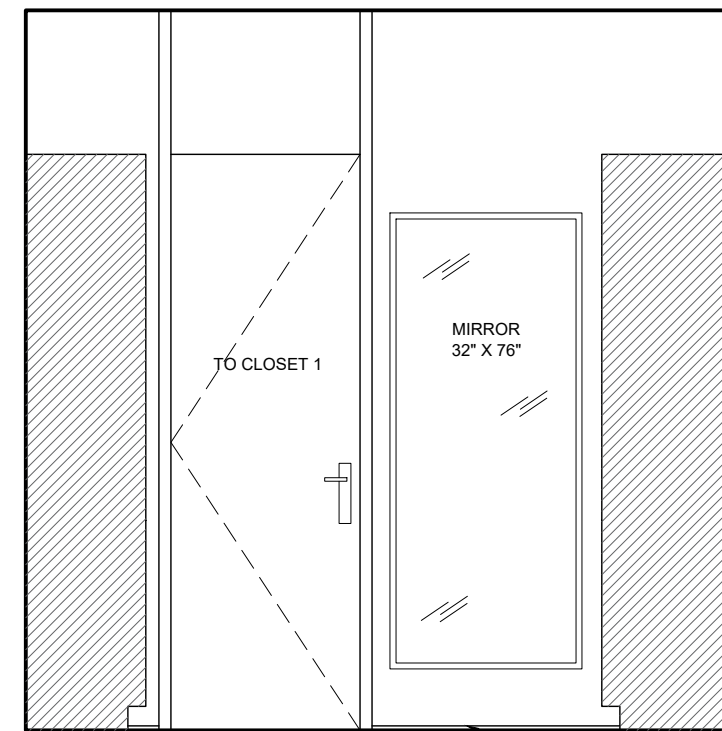
113 W.I.C 2 - ELEVATION C
