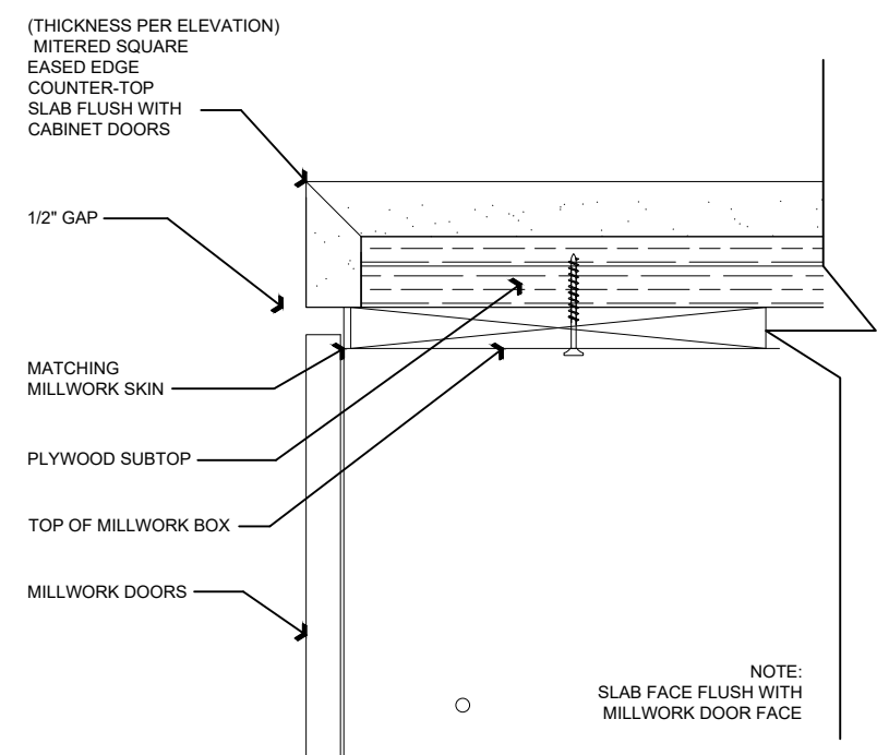
COUNTERTOP EDGE WITH MILLWORK REVEAL
