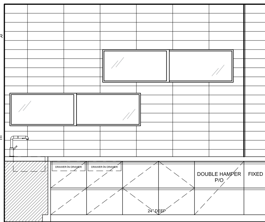
116 LAUNDRY - ELEVATION B
