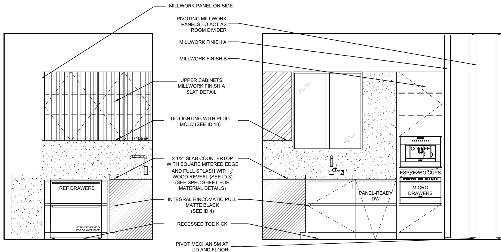
204 VIEWING LOFT - ELEVATION A
