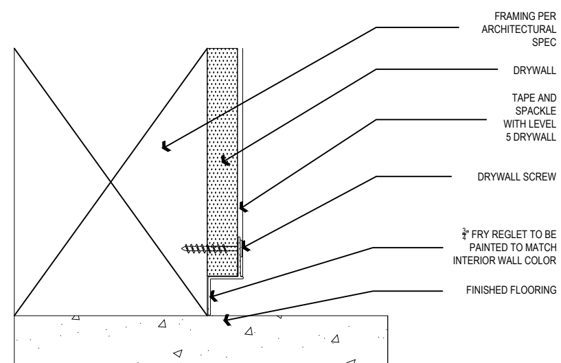
(TYP) 3/4" REGLET RECESSED BASE
