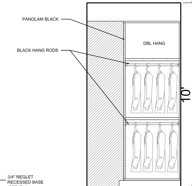
115 W.I.C 3 - ELEVATION D
