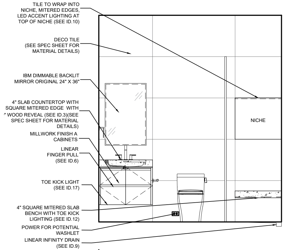
118 CASITA BATH - ELEVATION A
