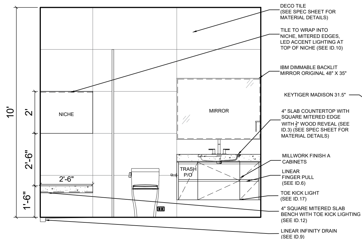
110 BATH 1 - ELEVATION A
