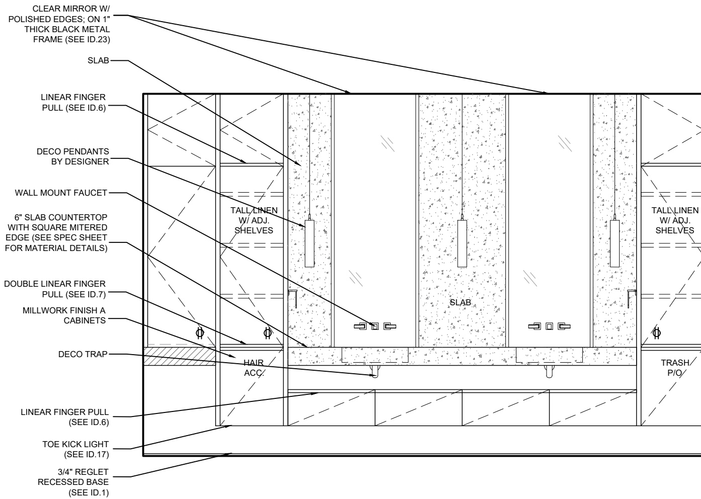
202 MASTER BATH - ELEVATION A
