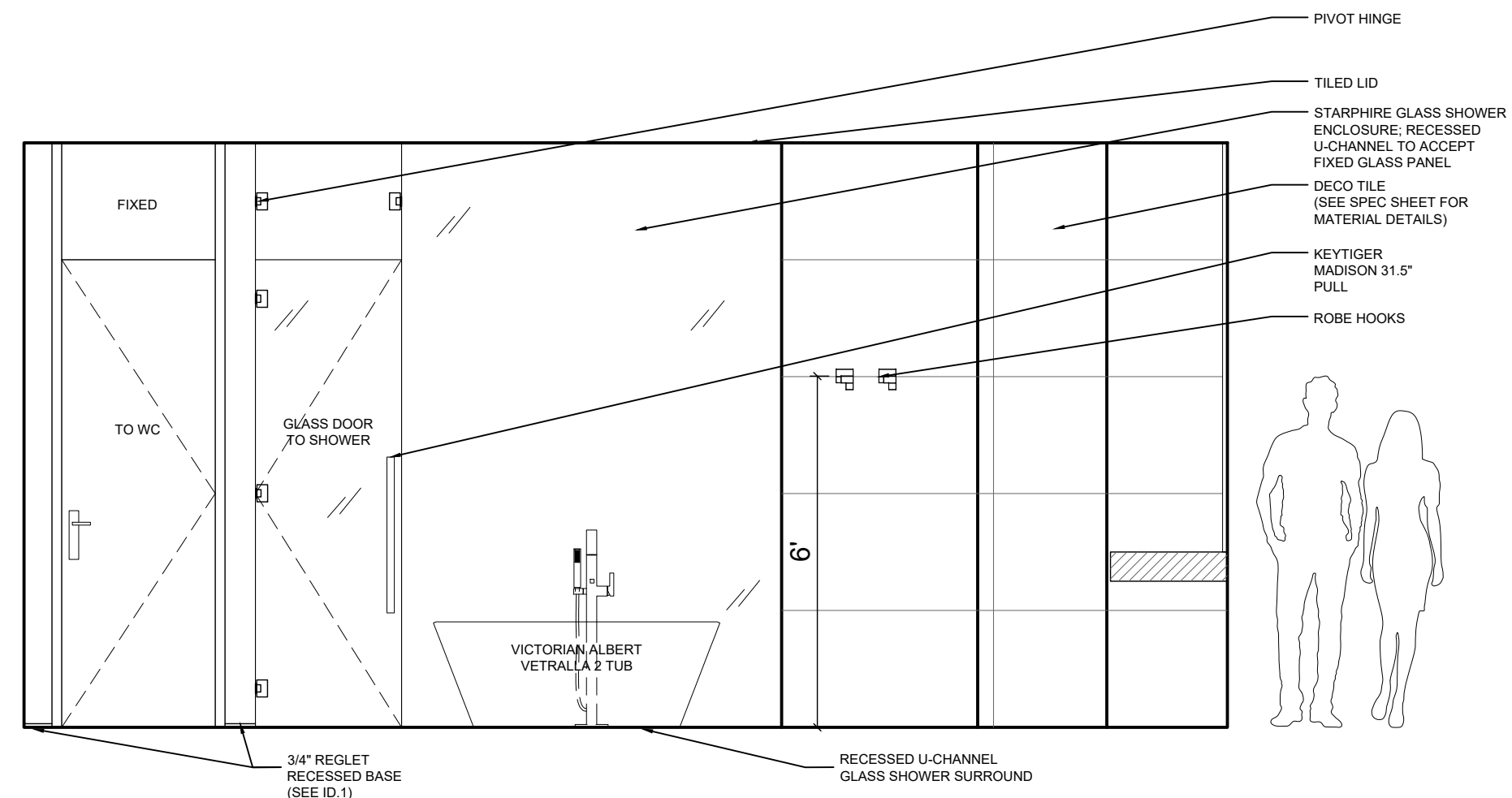
202 MASTER BATH - ELEVATION C
