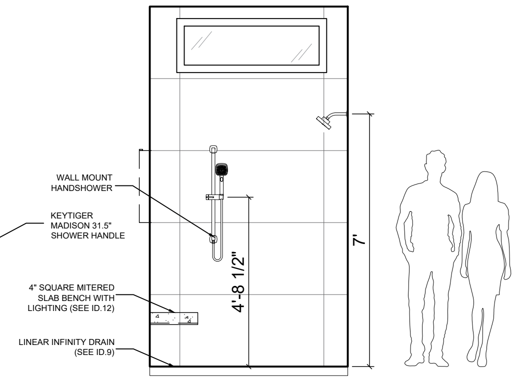
112 BATH 2 - ELEVATION B.1
