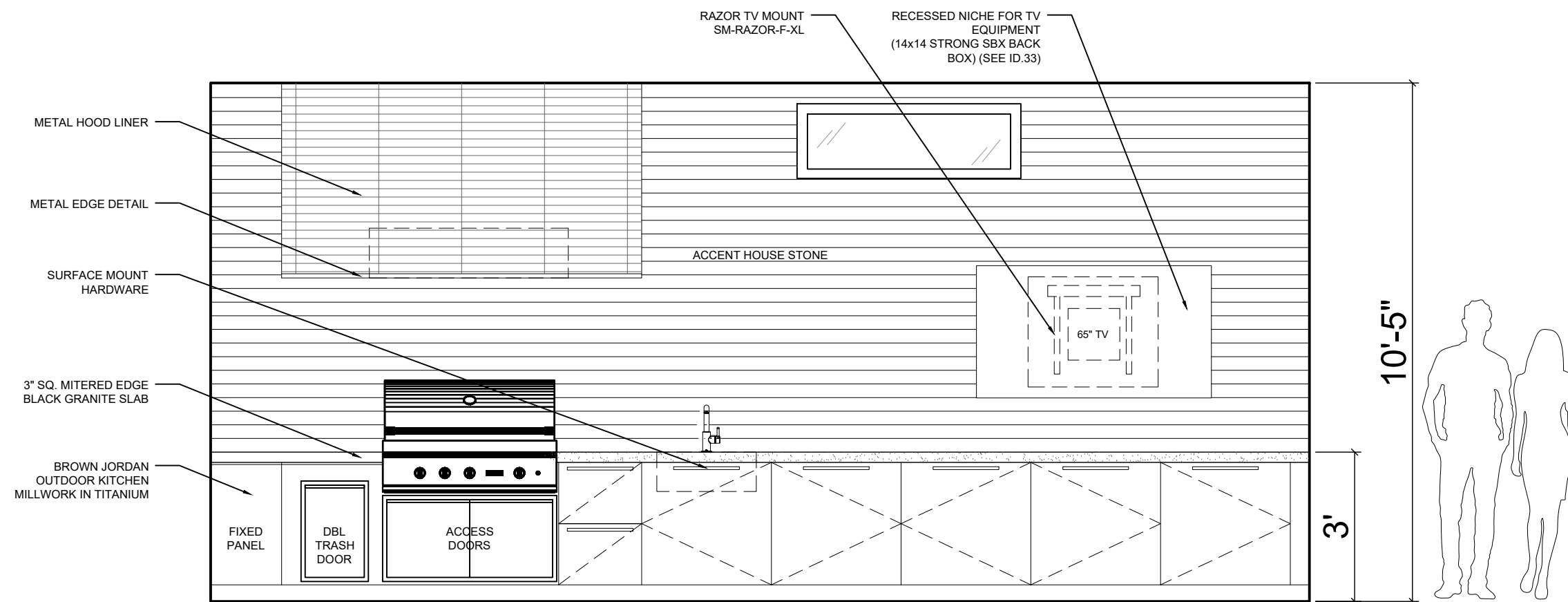
119 BBQ - ELEVATION A
