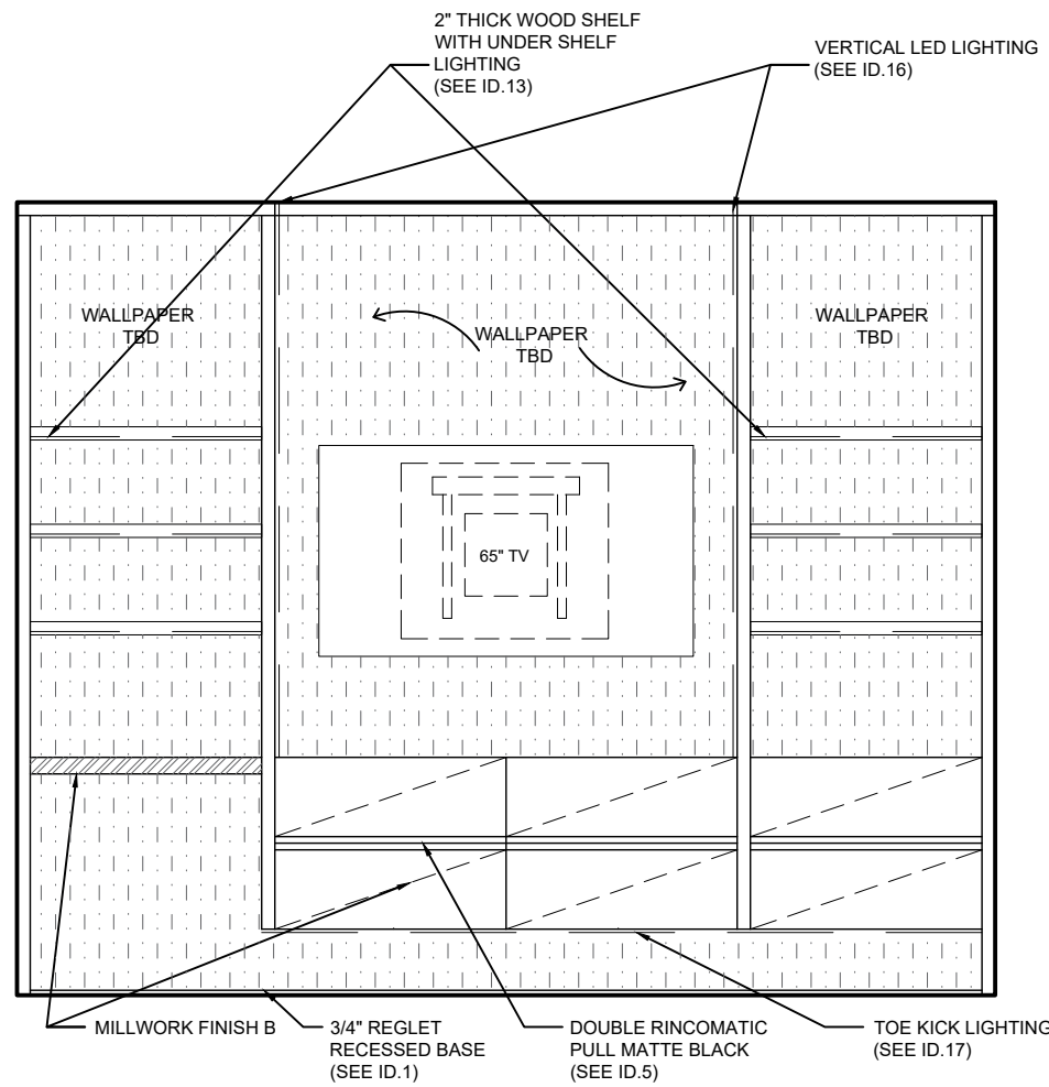
106 BONUS ROOM (OPEN) - ELEVATION A
