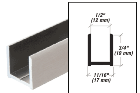
US HORIZON METAL U-CHANNEL (RECESSED FOR 1/2" FIXED GLASS PANELS) AU-HP12-MB FINISH: MATTE BLACK
