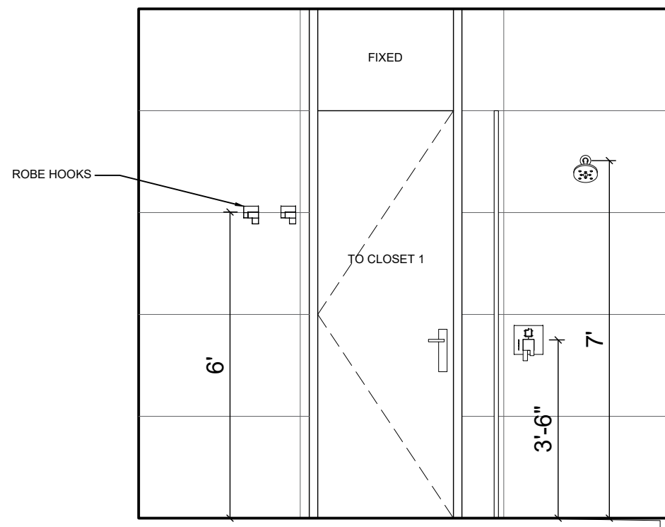
110 BATH 1 - ELEVATION C
