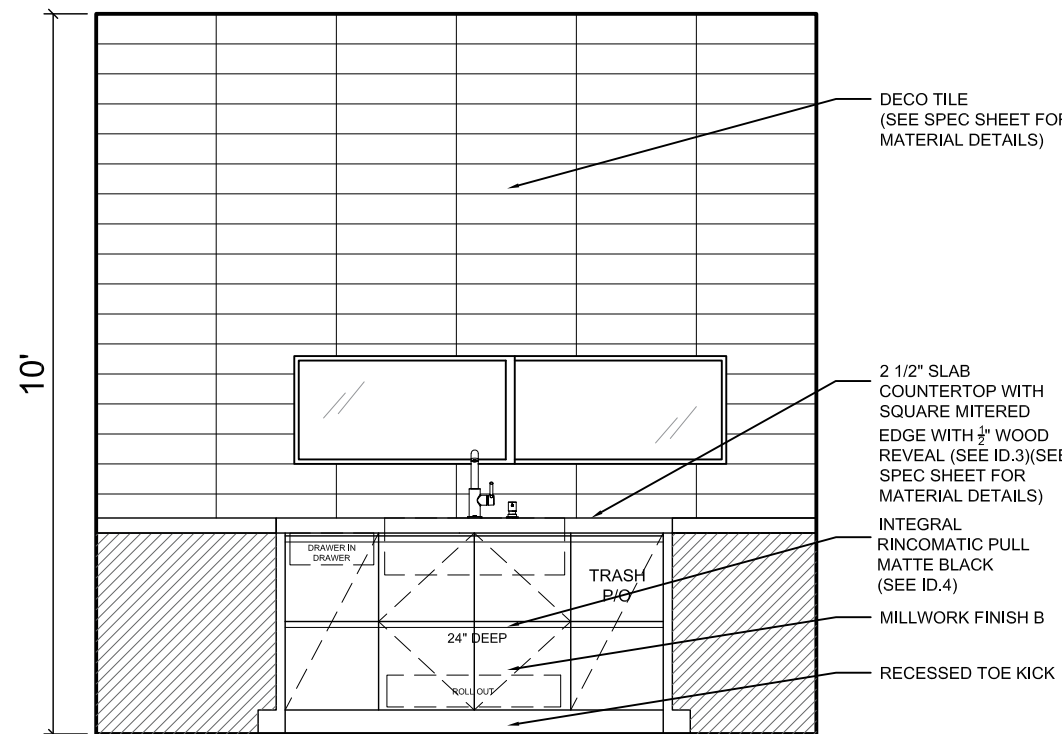
116 LAUNDRY - ELEVATION A
