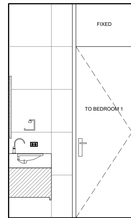
110 BATH 1 - ELEVATION D
