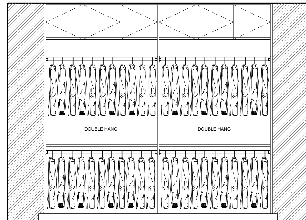
203 MASTER W.I.C - ELEVATION B
