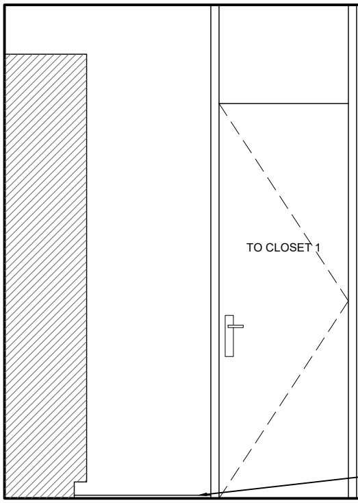
111 W.I.C 1 - ELEVATION C
