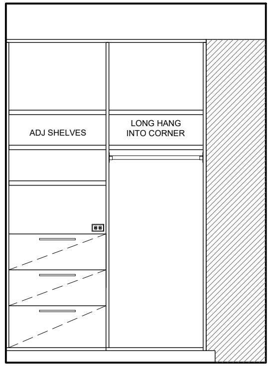
111 W.I.C 1 - ELEVATION A
