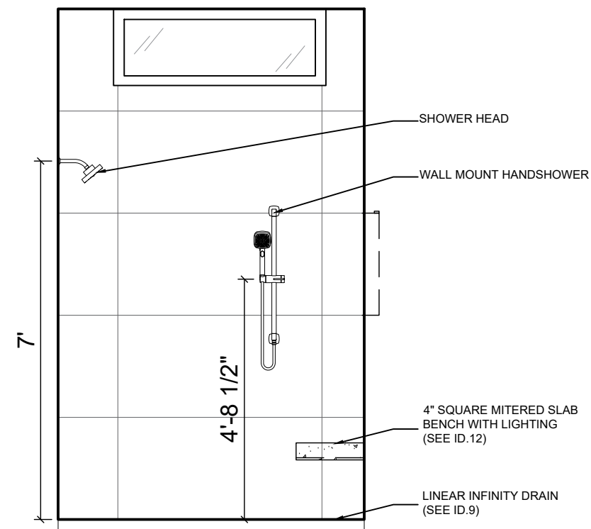
110 BATH 1 - ELEVATION B.1
