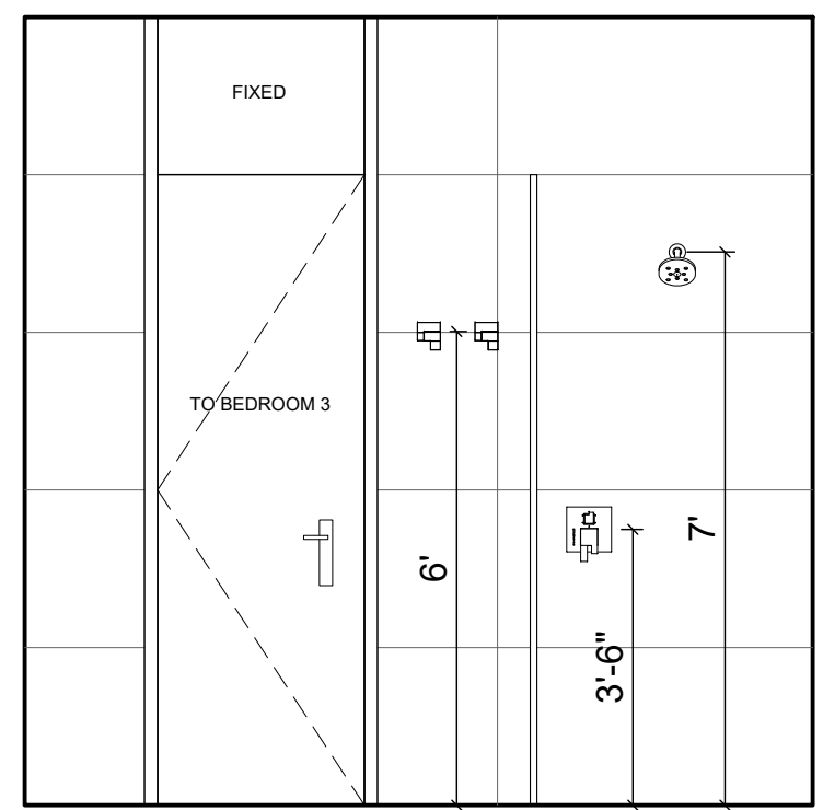
114 BATH 3 - ELEVATION C
