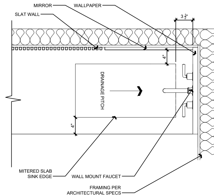
INTEGRAL SLAB SINK (PLAN)
