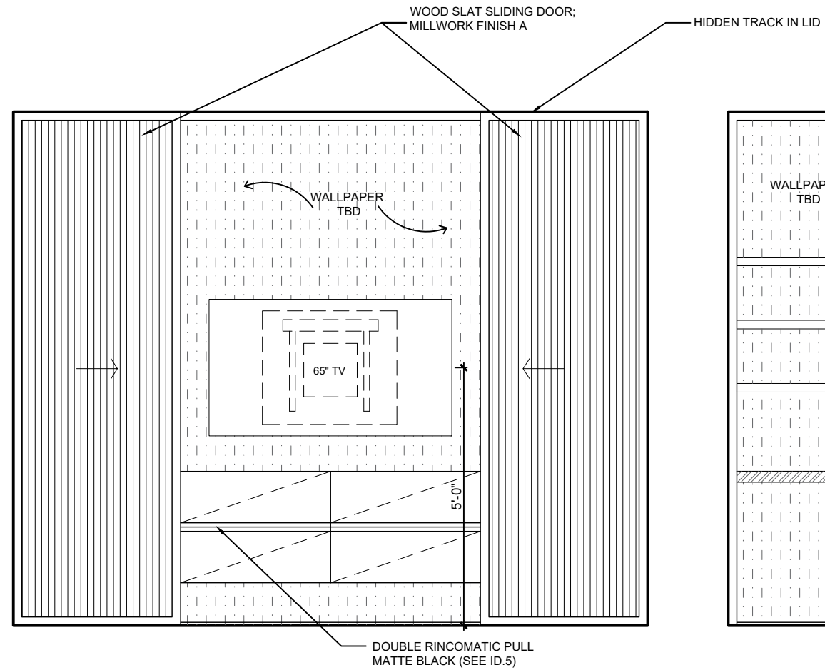
106 BONUS ROOM (OPEN) - ELEVATION A
