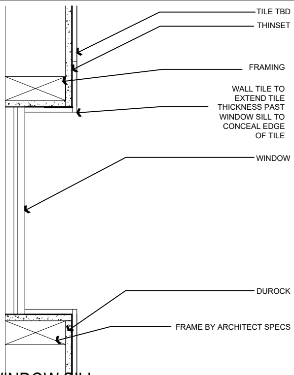
TILED WINDOW SILL
