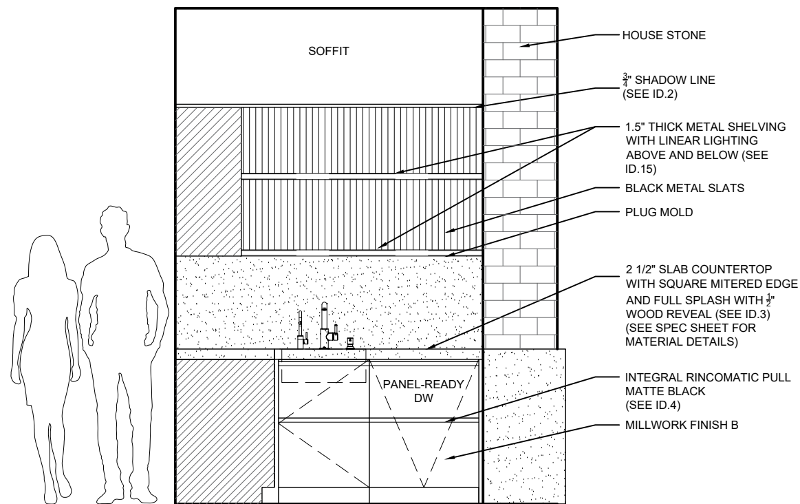
104 BAR - ELEVATION A
