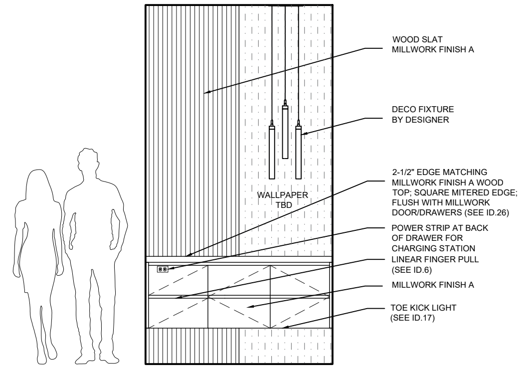
201 MASTER BEDROOM ELEVATION B
