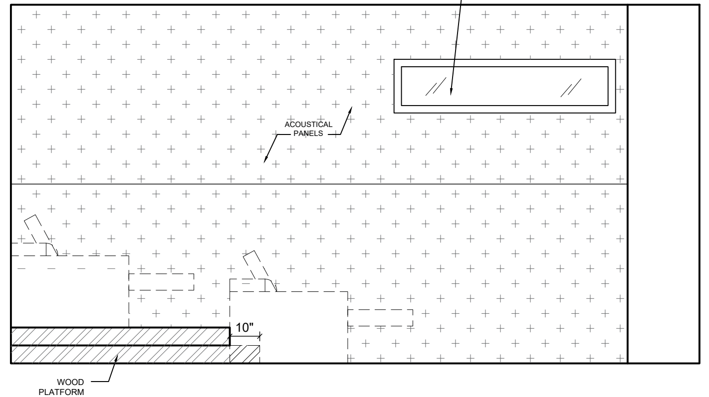
107 THEATER - ELEVATION D
