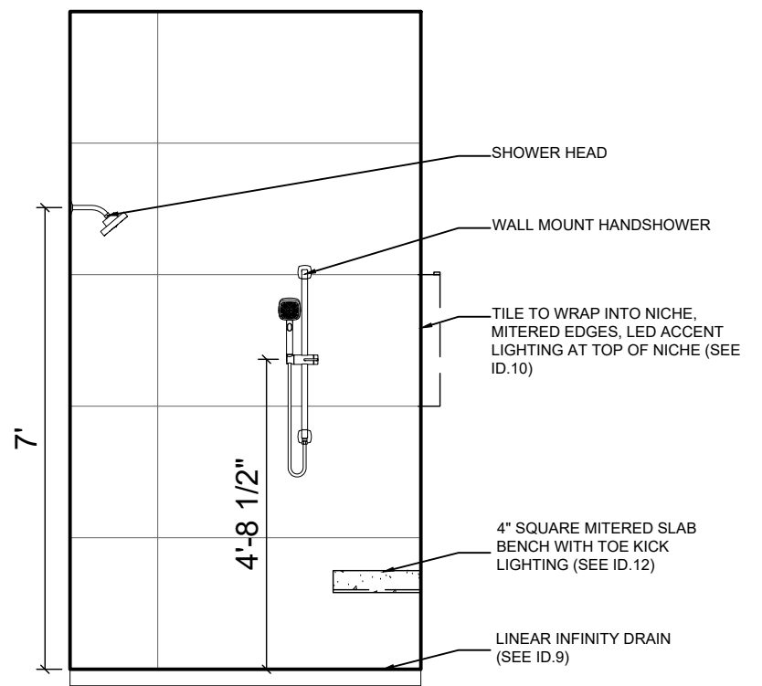
114 BATH 3 - ELEVATION B.1
