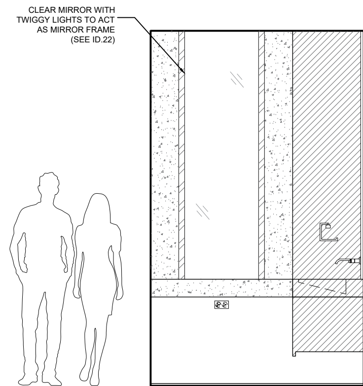
202 MASTER BATH - ELEVATION B
