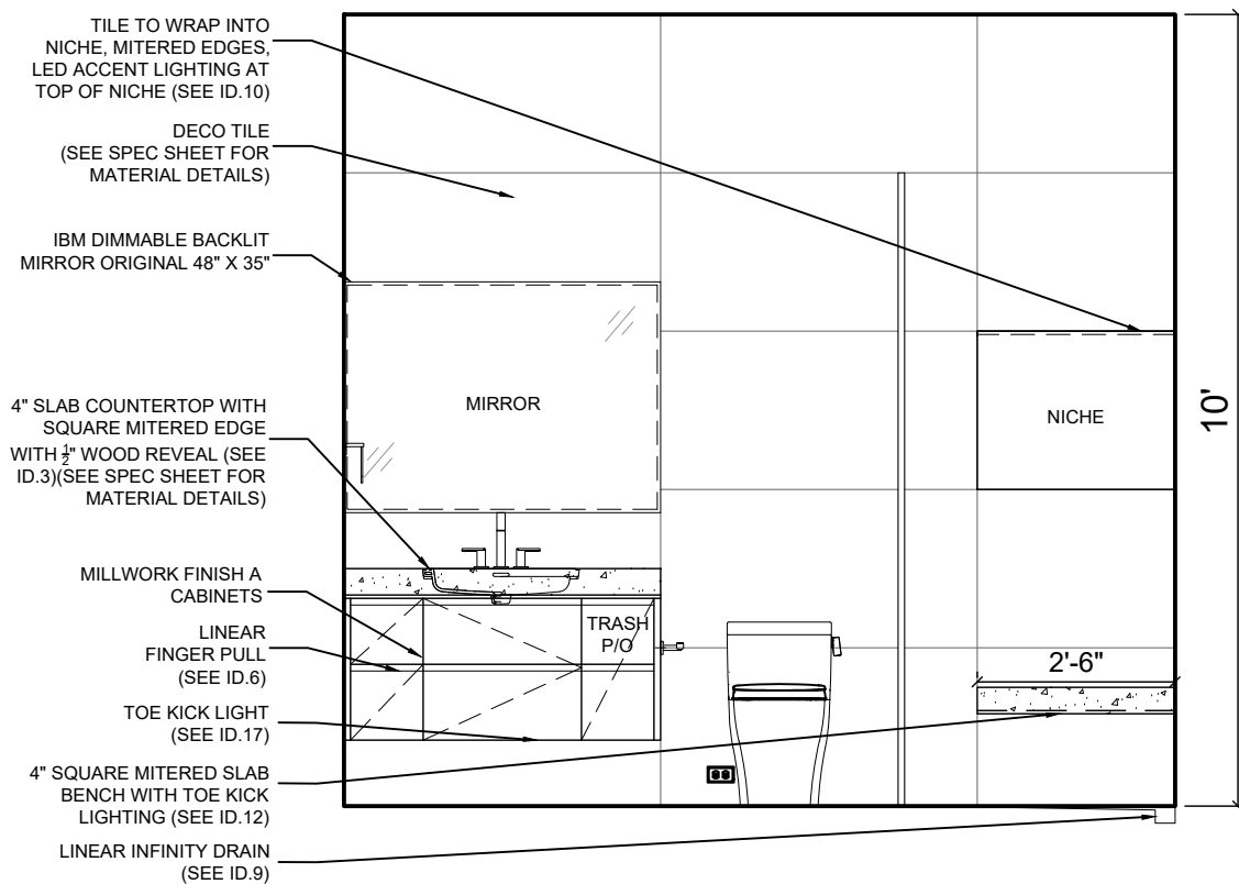
112 BATH 2 - ELEVATION A
