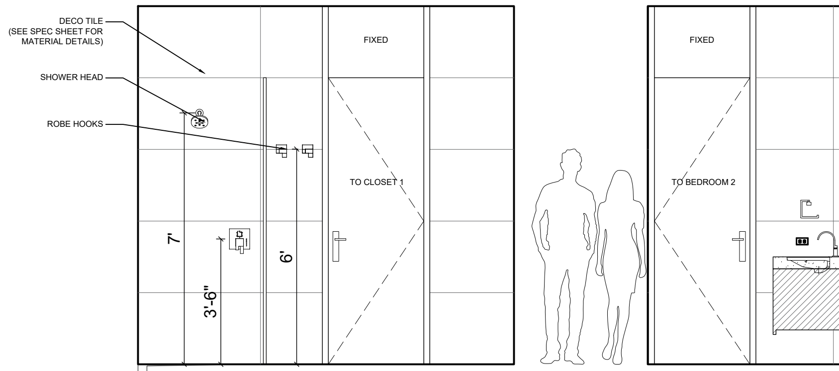
112 BATH 2 - ELEVATION C
